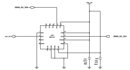
3-AXIS/MAGNETIC SENSOR
