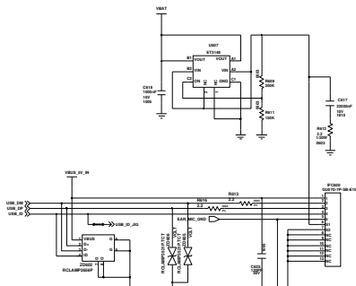
Micro USB Connector
