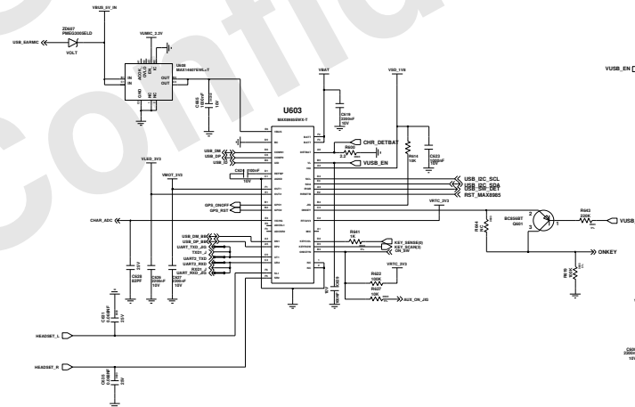
USB/CHARGE SWITCH
